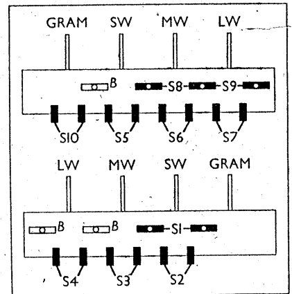
Diagrams of both sides of the switch unit. The upper one shows the switches seen from the underside of the chassis, while the lower one shows those on the side facing the chassis deck.
